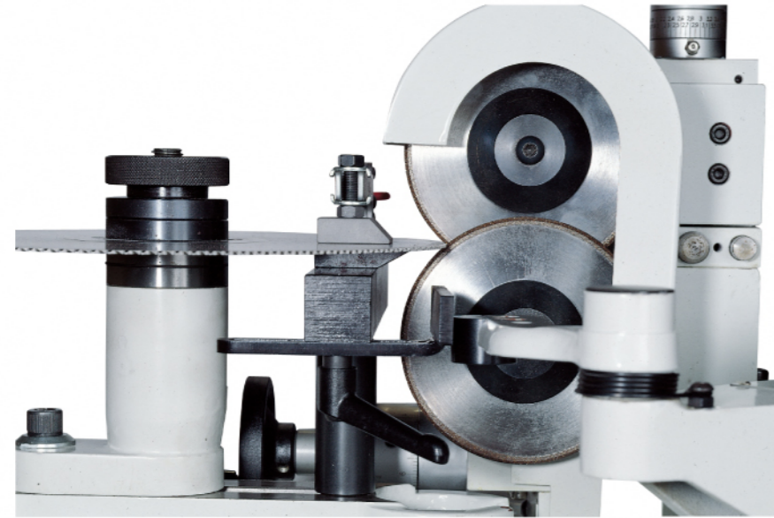
S500L Grinding Wheel Thickness Adjusting Scale 砂輪厚度調整刻度
